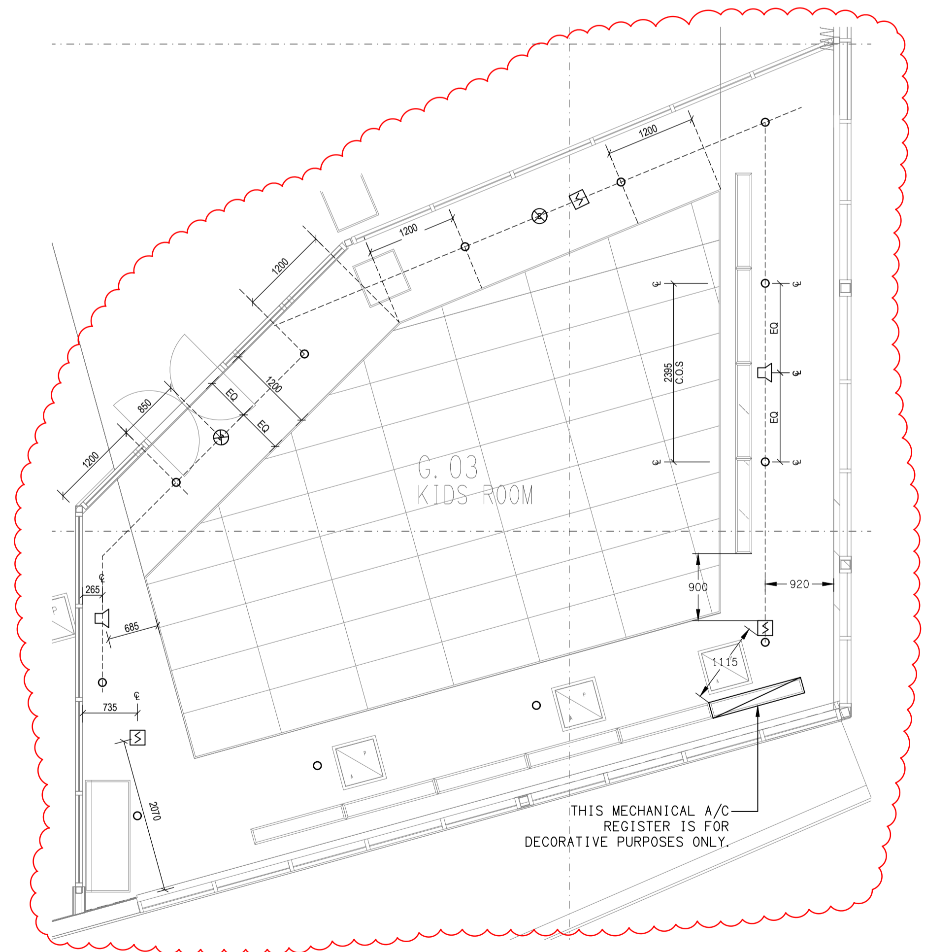
DETAIL A KIDS ROOM CEILING LAYOUT SCALE 1:50
